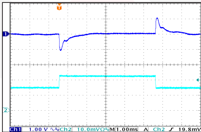
Figure 11: Output Voltage Response to Step-Change in Load Current , (50%-75%-50% of Iout(max); di/dt = 2 A/ \mu s). Load capacitance: 1 \mu F ceramic and 100 \mu F electrolytic capacitors. Ch 1: \Delta Vout (1 V/div); Ch 2: Iout (5 A/div). Timescale: 1ms/div.
