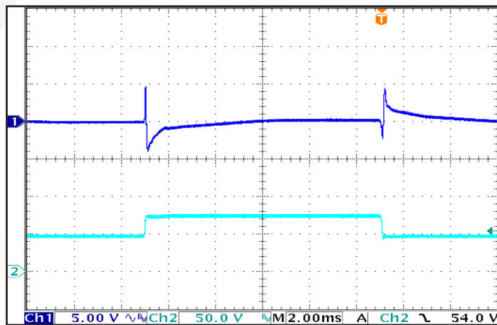
Figure 12: Output Voltage Response to Step-Change in Input Voltage , (dV/dt = 250 V/ms). Load capacitance: 1 \mu F ceramic and 990 \mu F electrolytic capacitors. Ch 1: Vout (5 V/div); Ch 2: \Delta Vin (50 V/div). Timescale: 2ms/div
