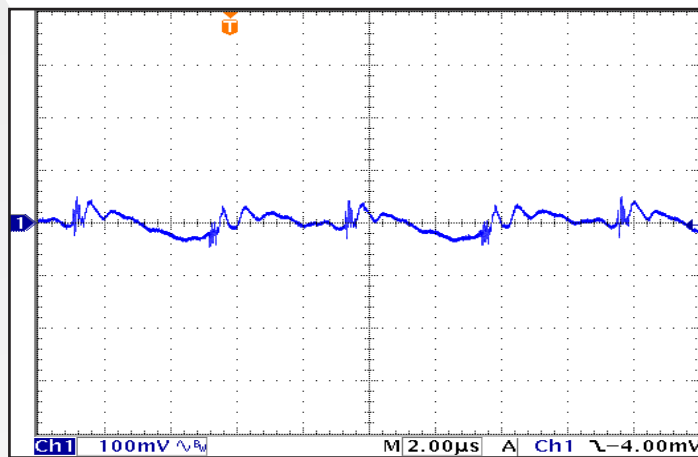
Figure 10: Output Voltage Ripple , Vout, at nominal input voltage and rated load current (100 mV/div). Load capacitance: 1 \mu F ceramic and 100 \mu F electrolytic capacitors. Bandwidth: 20 MHz. See Figure 13. Timescale: 2 \mu s/div.
