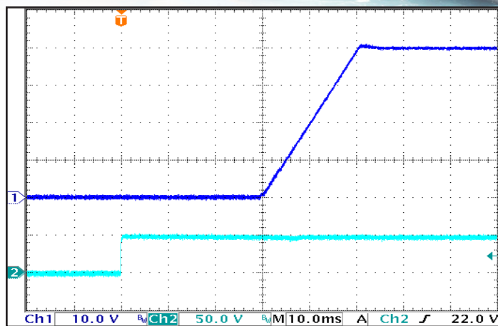
Figure 8: Turn-On Transient , at full resistive load and zero output capacitance, initiated by Vin. Ch 1: Vout (10 V/div); Ch 2: Vin (50 V/div). Timescale: 10ms/div.
