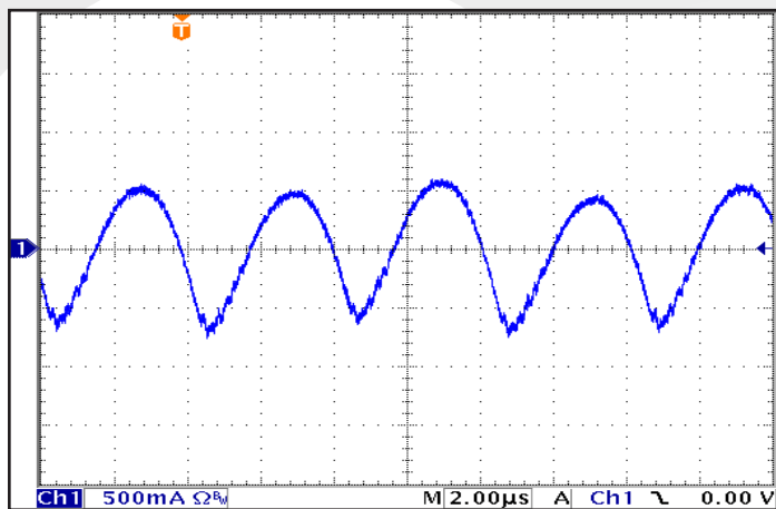
Figure 9: Input Terminal Current Ripple , i_c , at full rated output current and nominal input voltage with a 220 \mu F electrolytic capacitor (500 mA/div). Bandwidth: 20 MHz. See Figure 13. Timescale: 2 \mu s/div.
